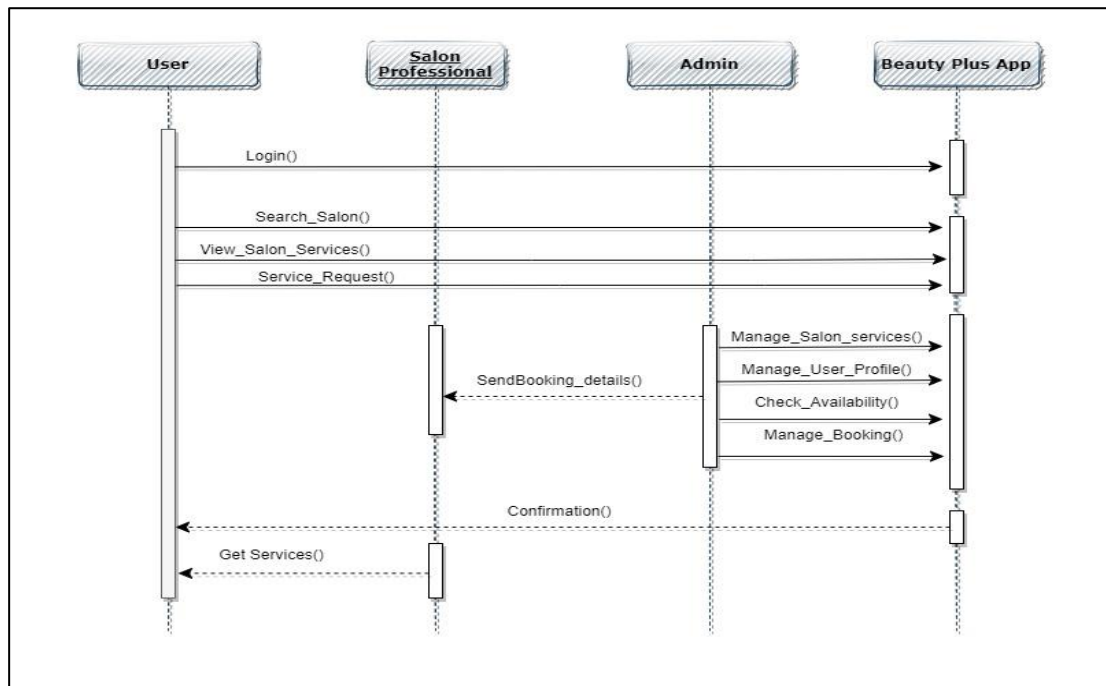
Figure 2Sequence Diagram
