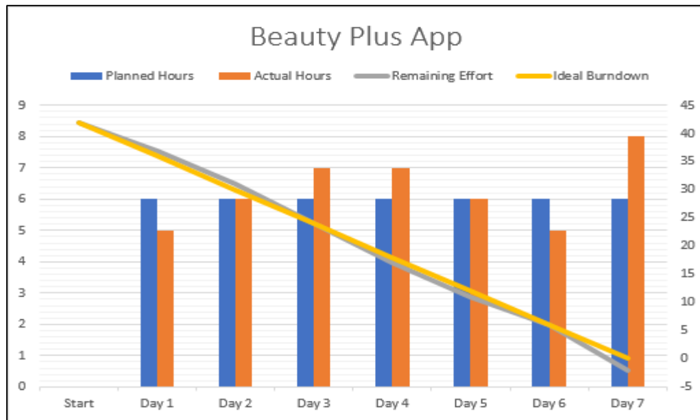
Figure 21 Burn-Down Chart for Sprint 1
