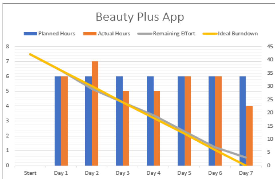
Figure 22 Burn-Down Chart for Sprint 2
