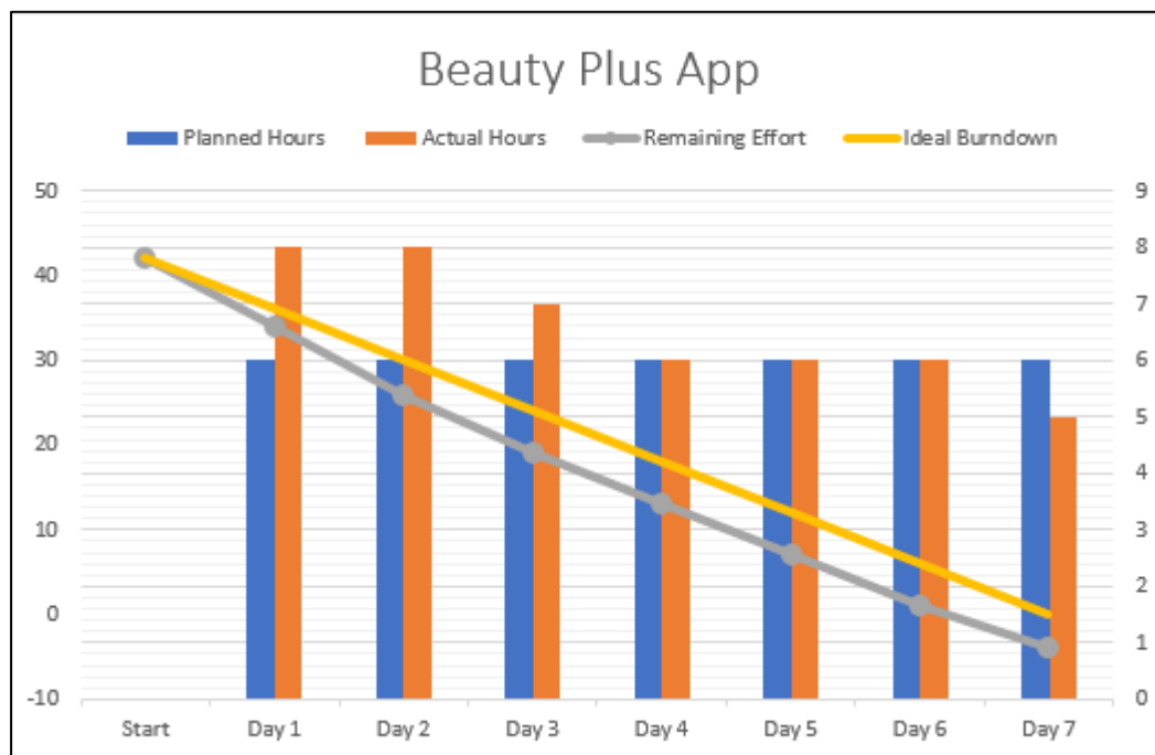
Figure 24 Burn-Down Chart for Sprint 4
