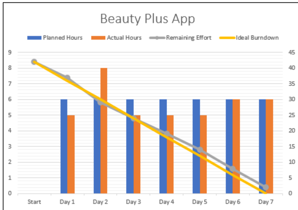
Figure 23 Burn-Down Chart for Sprint 3
